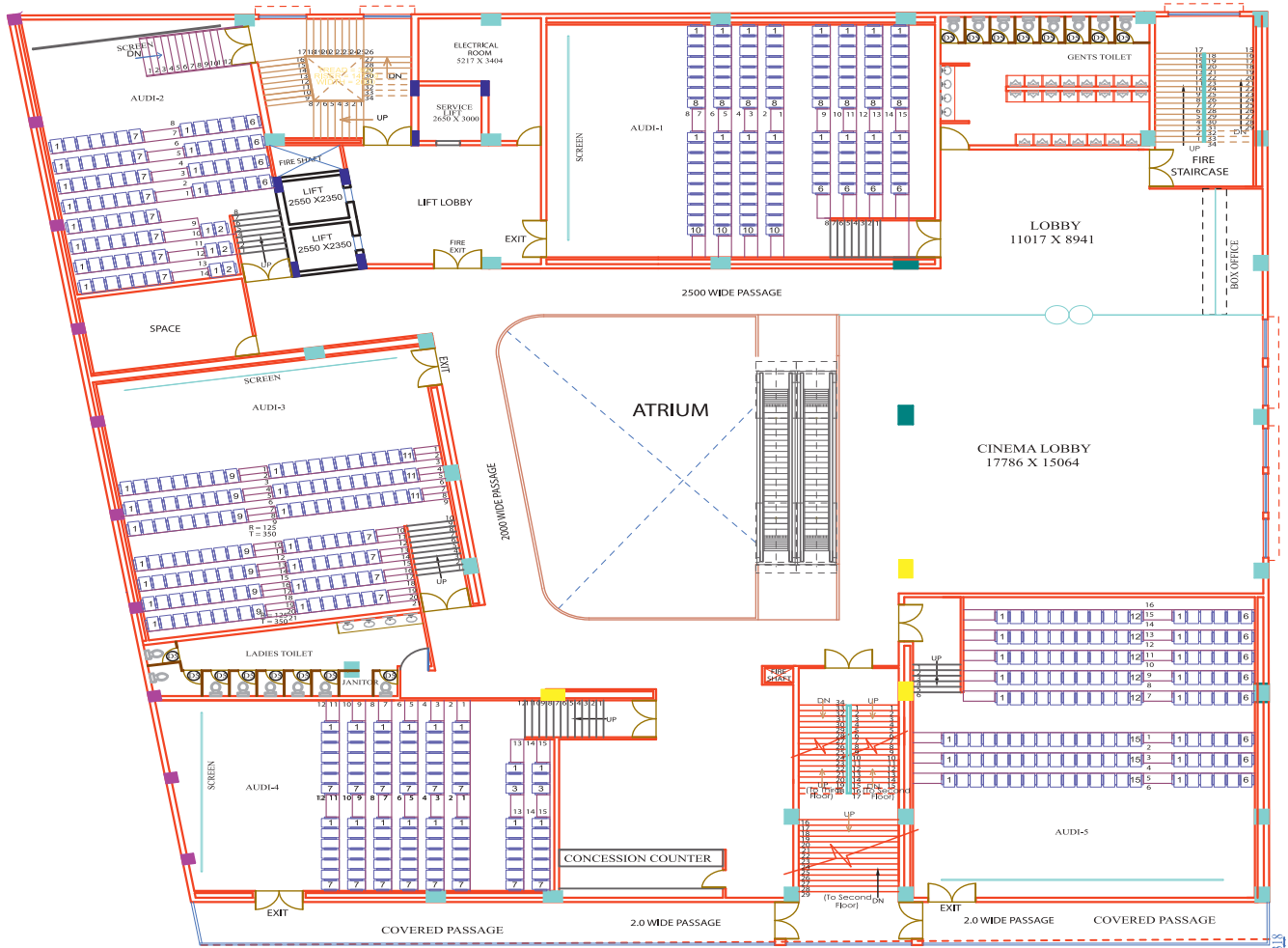
THIRD FLOOR PLAN (MULTIPLEX LVL.)
